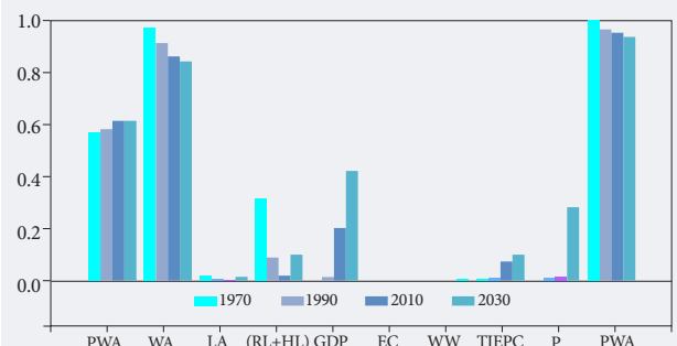
Figure 4. Tibet Analysis for the Period 1978-2018
